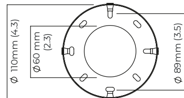
mounting plate dimensions 240V
