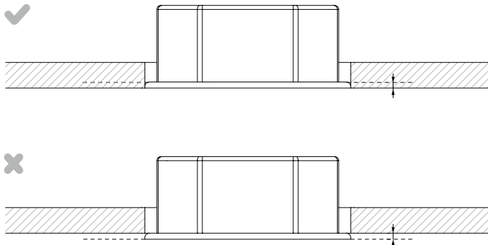
Top view of J-box and UMP
