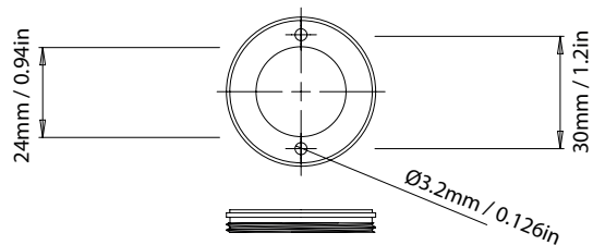
Mounting plate
